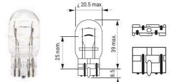
8 W21/5W BASE W3x16q
