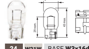
24 W21W BASE W3x16d
