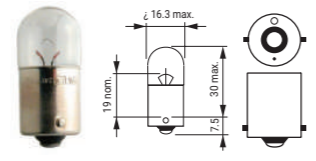
11 R10W BASE BA15s
