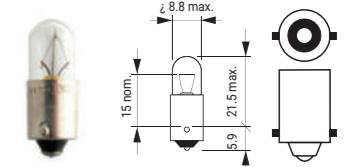
9 T4W BASE BA9s
