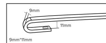
U-HOOK WIPER BLADE ARMS: 9mm*11mm
