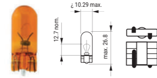
26 WY5W BASE W2.1x9.5d
