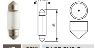
17 C5W BASE SV8.5
