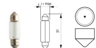
4 T10X31 BASE SV8.5
