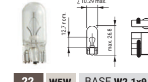
22 W5W BASE W2.1x9.5d
