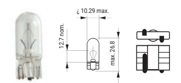
6 W5W BASE W2.1x9.5d
