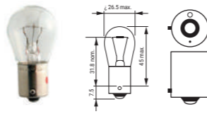
12 P21W BASE BA15s
