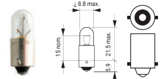
27 T4W BASE BA9s
